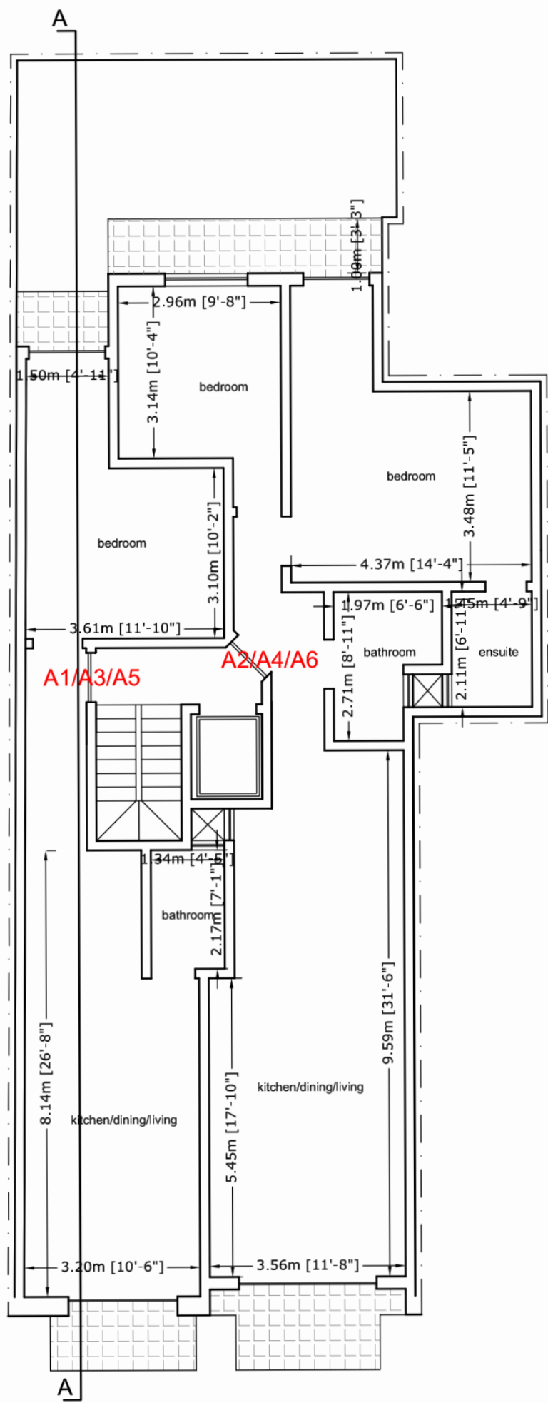
Proposed 1st, 2nd, 3rd Floor Plan
