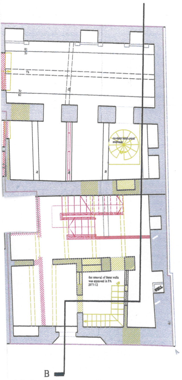
existing/ proposed ground floor - scale 1:100
