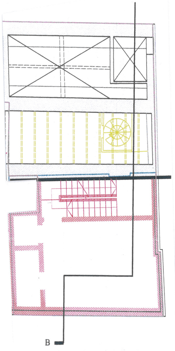
existing/ proposed lower first floor - scale 1:100
